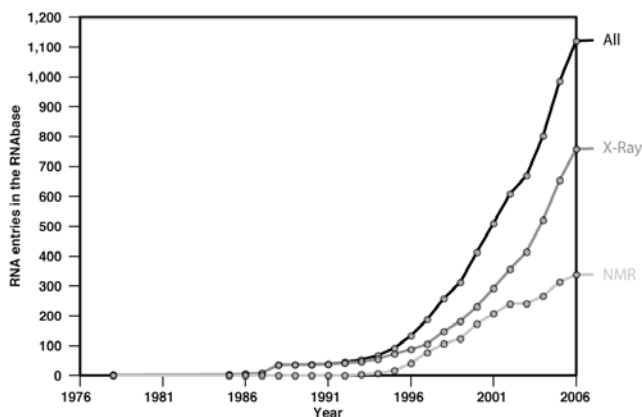
Fig. (1). Yearly growth of RNA structure deposition in the RNA-base database. Black curve shows all entries in the RNABase, dark-grey curve shows only entries that were determined by X-Ray experiments and light-grey curve shows those determined by Nuclear Magnetic Resonance experiments.
