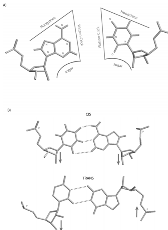
Fig. (2). Base-pair interactions. A) Watson-Crick (WC), Hoogsteen and sugar edges for a base-pair interaction. B) cis and trans states of a base-pair interaction.
