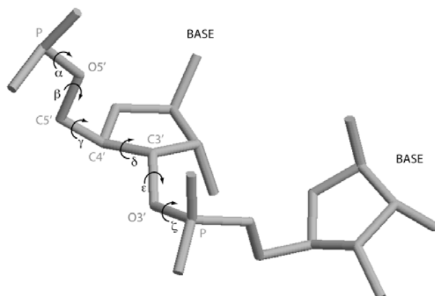
Fig. (4). RNA Backbone torsion angles.
